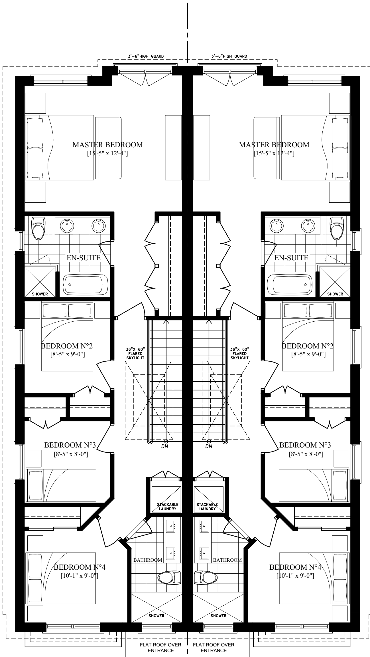
2ND FLOOR PLAN PLAN NOT TO SCALE
